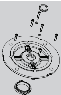
Brida FF
