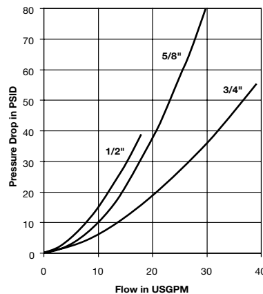
Performance FEC Series (1/2", 5/8", 3/4") Test Fluid: Oil - 200 SUS
