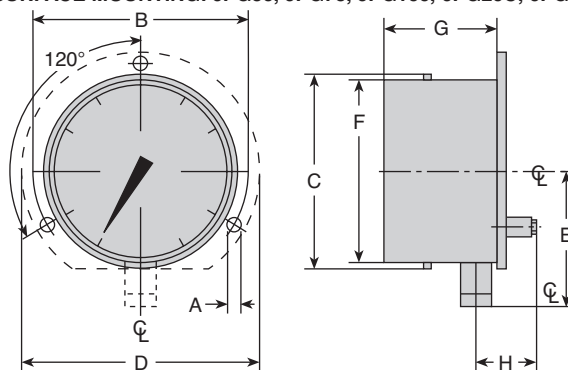
SURFACE MOUNTING: 6PG50, 6PG75, 6PG100, 6PG20C, 6PG30C
