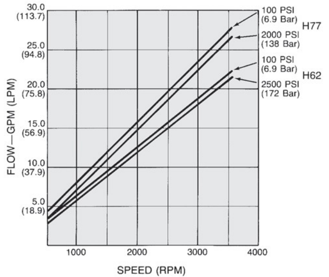
H62/H77 Flow/Speed
