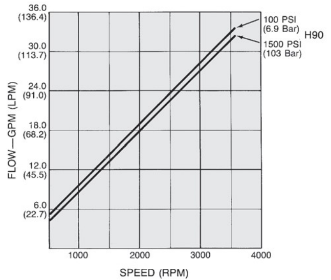
H90 Flow/Speed
